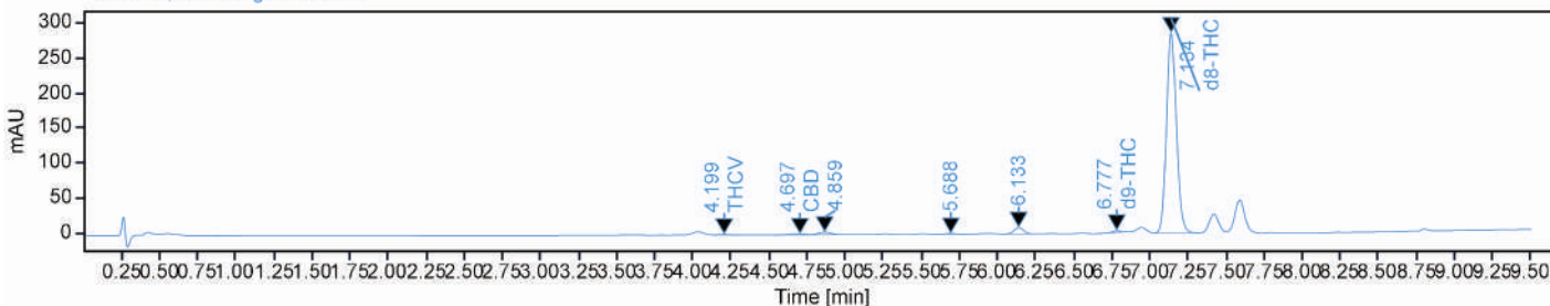
VWD1A, Wavelength=230 nm
